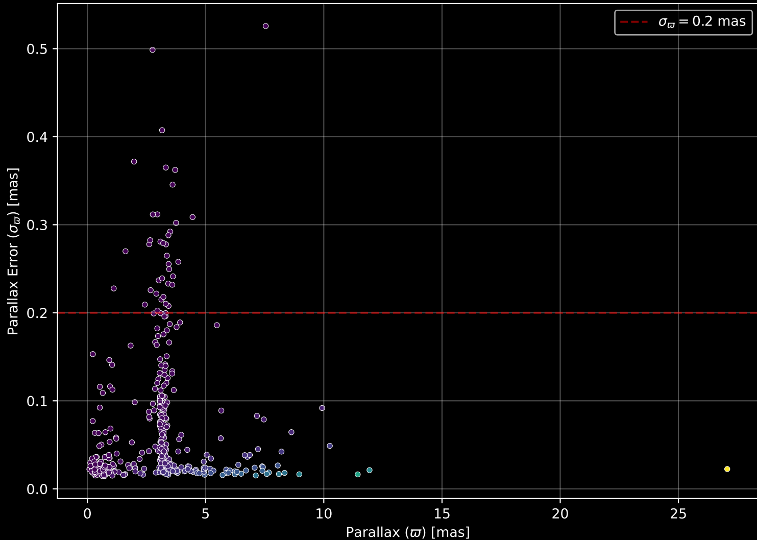
APOGEE DR17 Field: [IC348] Parallax Quality (n= 381)
