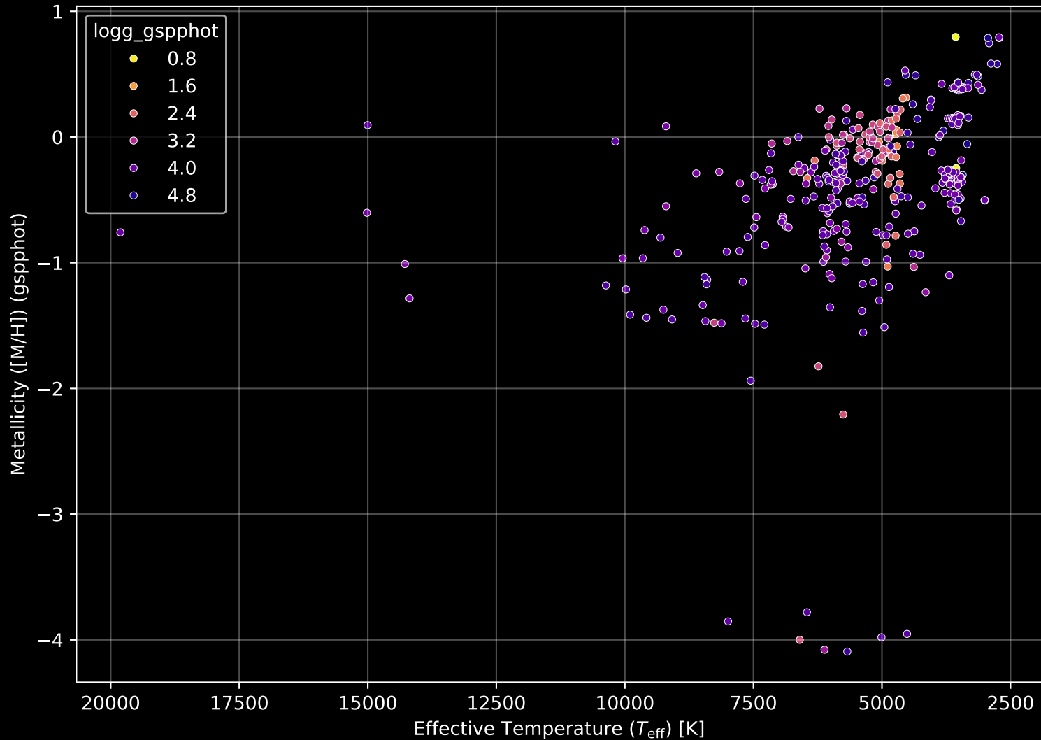
APOGEE DR17 Field: [IC348] Stellar Population Parameters (n= 381)
