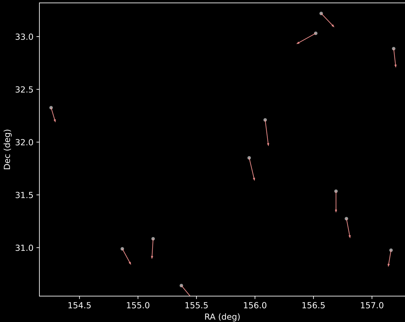
APOGEE DR17 Cluster 7 Proper Motion Vectors (n=12)
