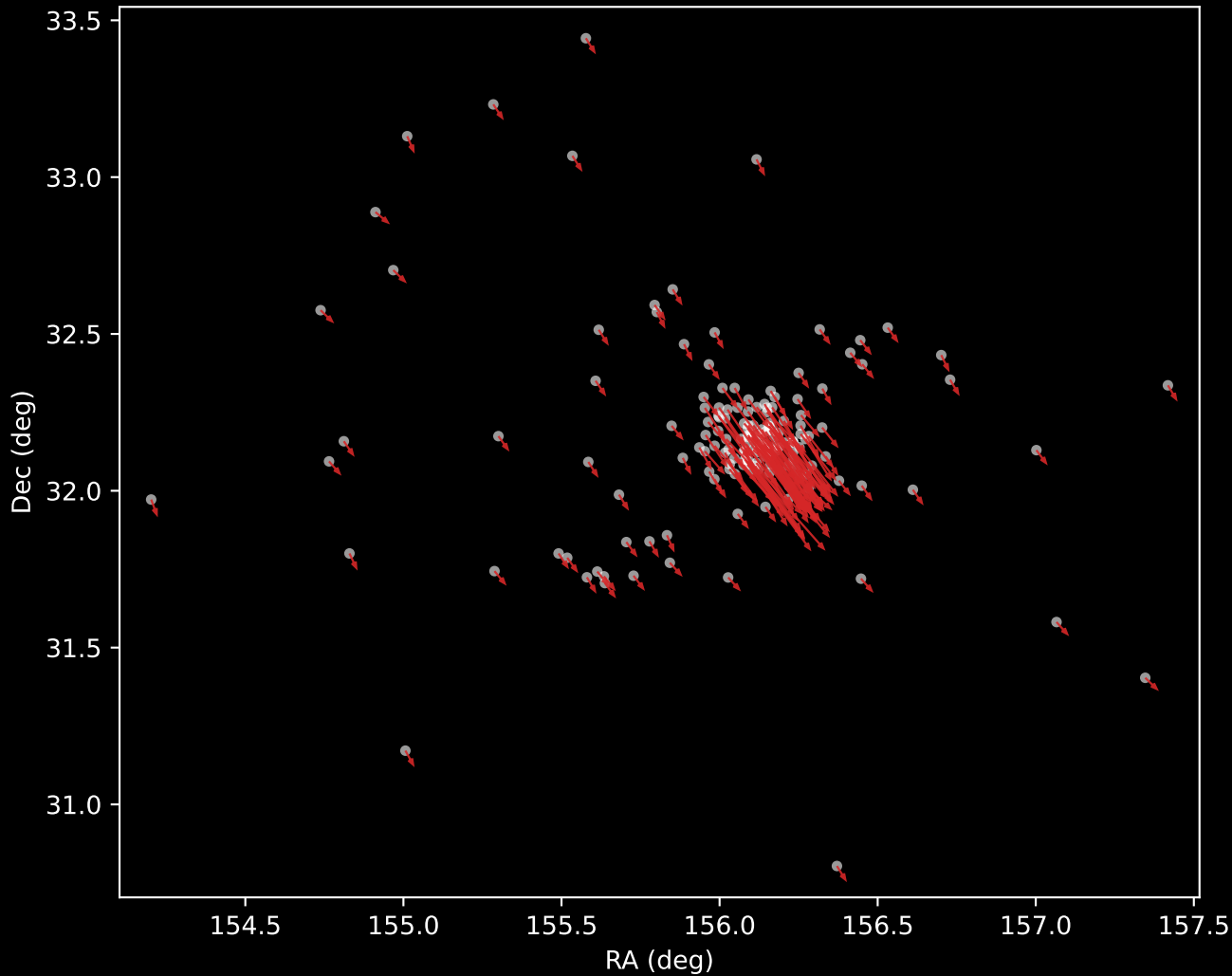
APOGEE DR17 Cluster 6 Proper Motion Vectors (n=170)
