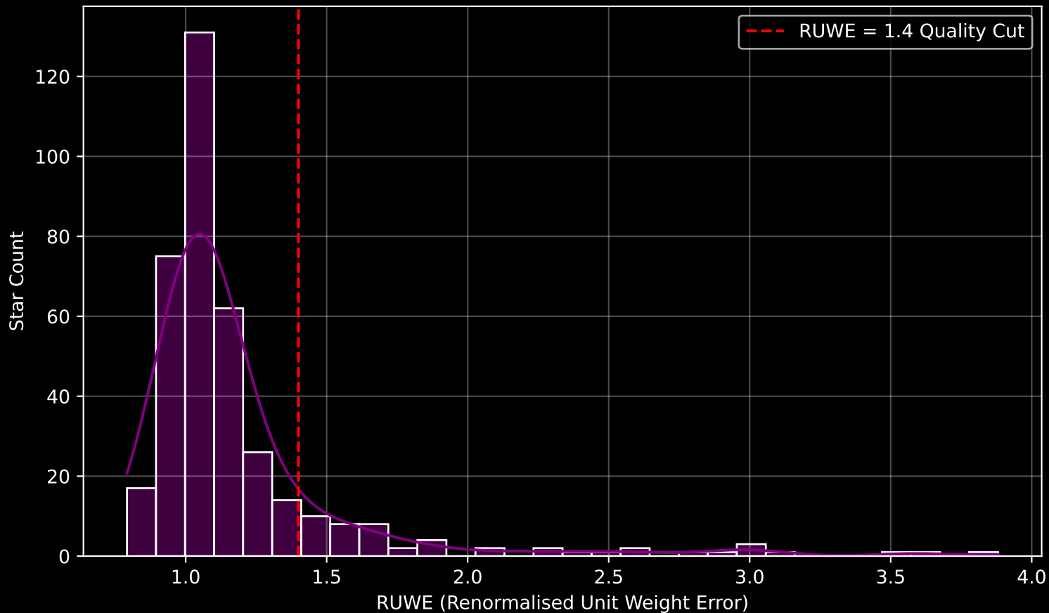
GAPOGEE DR17 Field [IC348] RUWE Distribution (n= 374)
