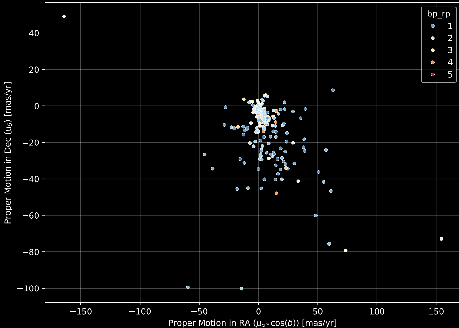
APOGEE DR17 Field: [IC348] Proper Motion Diagram (n= 381)
